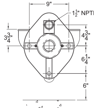
R2100-W-1 SHOWN
